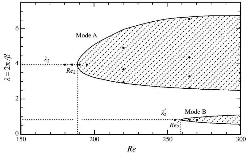
FIGURE 1. Curves of neutral stability for the two-dimensional Kármán vortex street with respect to spanwise perturbations. Linearly unstable modes exist everywhere inside the shaded regions. The upper region corresponds to a family of long-wavelength instabilities with critical values Re_2 \simeq 190 , \lambda_2 \simeq 3.96d ; the lower region corresponds to a family of short-wavelength instabilities with critical values Re'_2 \simeq 260 , \lambda'_2 \simeq 0.822d . Each point ( \bullet ) on this plot represents a three-dimensional mode considered in §3.
