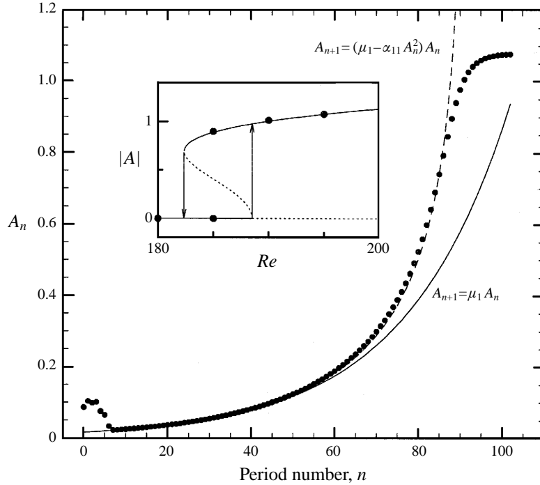
FIGURE 5. Nonlinear growth of a three-dimensional perturbation to the wake near the secondary instability threshold at Re_2 \simeq 190 , \lambda_2 = 3.96d : \bullet , values of the amplitude A_n evaluated from simulations of the full Navier–Stokes equations at Re = 195 ; curves show predictions from equation (3.5) truncated at first and third order with \mu_1 = 1.041 and \alpha_{11} = -0.116 . The inset shows a bifurcation diagram along with simulation results at nearby parameter values.
