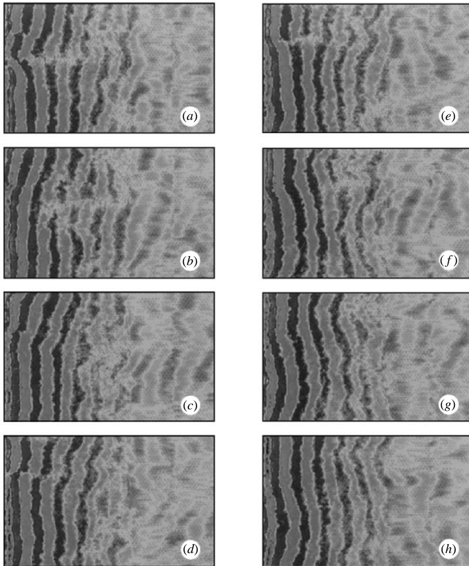
FIGURE 19. Visualization of the turbulent wake at Re = 1000 . The sequence of images ( a-h ) shows contours of the normal velocity v(x, y = 0, z, t) at times spaced approximately two shedding cycles apart. The image plane corresponds to x/d = (0, 48) and z/d = (0, 25.13) . The structures ‘wash out’ downstream because of the low resolution in that part the domain.
